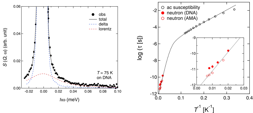
Fig. 1: (Left) QENS spectrum of Nd complex taken at 75 K using DNA spectrometer. (Right) Arrhenius plots of relaxation times obtained from QENS and ac susceptibility measurements.
