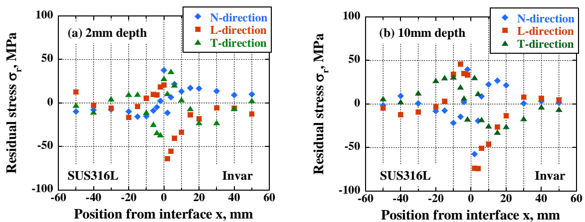
Fig. 1 Residual stress distributions of the Invar-SS316L HIP joint specimen measured using neutron diffraction at (a) 2 mm depth and (b) 10 mm depth.
