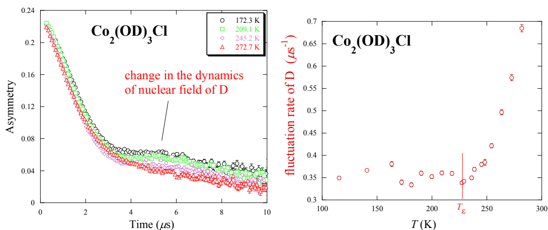
Fig. 1 Left: muon-spin-relaxation spectra indicating a change in the dynamics of D atoms in \text{Co}_2(\text{OD})_3\text{Cl} . Right: the analyzed fluctuation rate of D.
