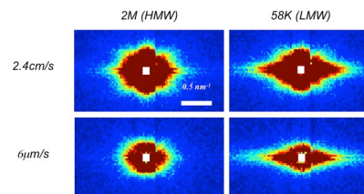
Figure 2. 2D SANS pattern from Blends of d-PE (Mw=600,000; 97%) and h-PE (Mw =2M, 58k; 3%) for two drawing rates (2.4 cm/s, 6 \mu\text{m/s} ).
