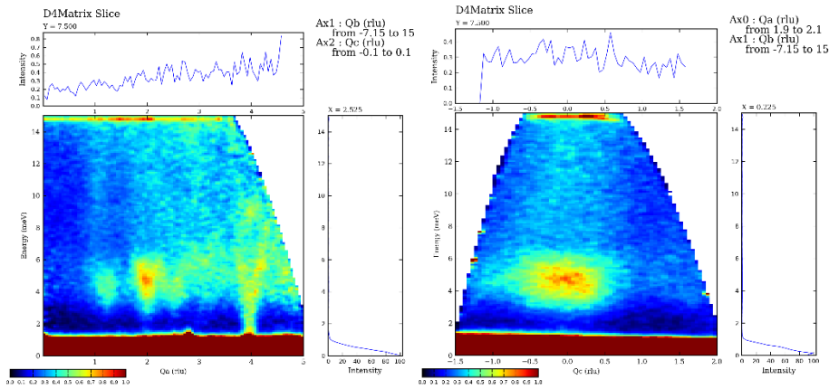
Figure 1. Scattering maps show magnetic excitations as a function of energy transfer and momentum transfer along [H,H] and [-H,H] directions
