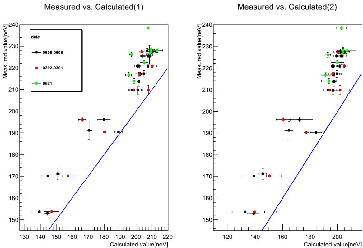
Figure 1: Comparison between measured (y-axis) and calculated (x-axis) Fermi potential. We have employed two different formula for the Fermi potential calculation. There are 20~30 neV discrepancy in each case. The reason is not clear and study is now under way.
