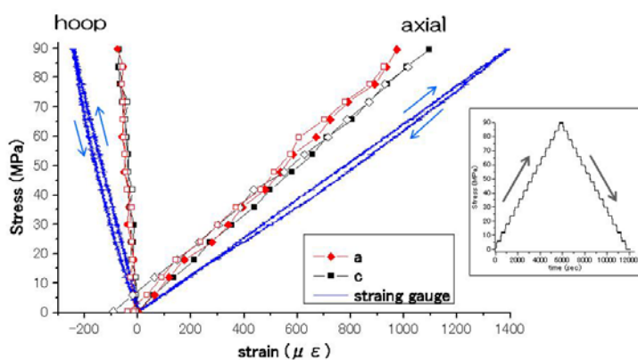
fig. 2. Stress-strain curves for Novaculite, and strain in a and c lattice parameters. The inset shows the novaculite loading sequence.
