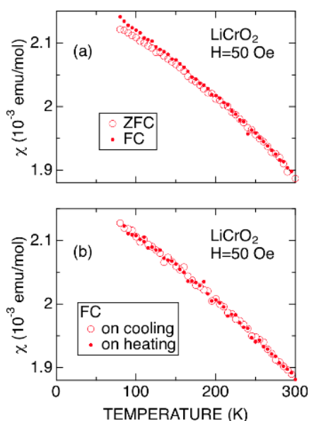
Fig.2 T dependences of \chi for \text{LiCrO}_2 ; (a) \chi obtained ZFC and FC mode and (b) \chi observed FC mode on heating and on cooling.
