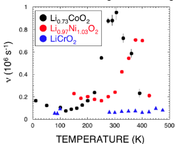
Fig.2 T dependences of \nu for \text{Li}_{0.73}\text{CoO}_2 , \text{Li}_{0.97}\text{Ni}_{1.03}\text{O}_2 and \text{LiCrO}_2 .
