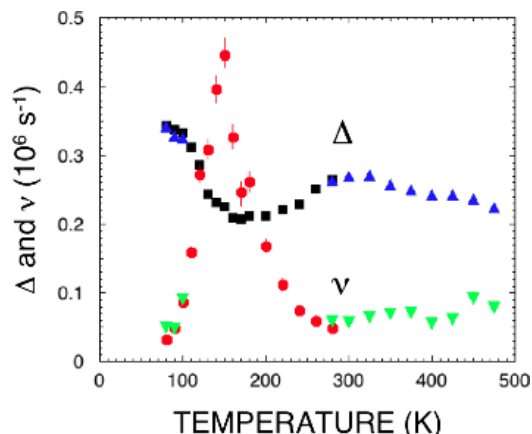
Fig.1 T dependences of \Delta and \nu for \text{LiCrO}_2 .
