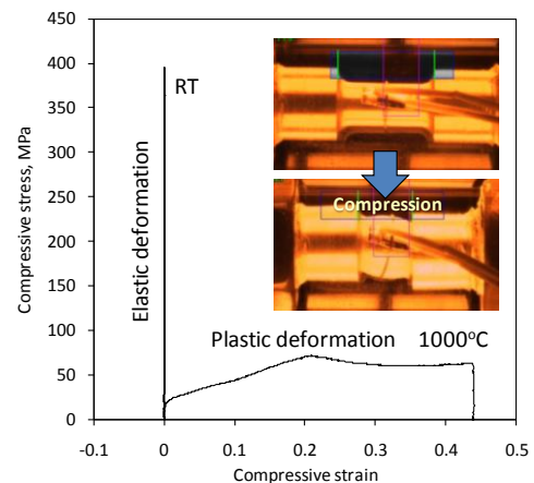
Fig.3 Relationship between compressive applied stress and macroscopic strain at RT and 1000°C.
