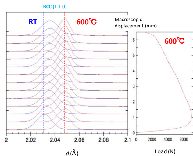
Fig.4 peak shifts of 110 reflection and change in macroscopic displacement at 600°C as a function of applied stress.
