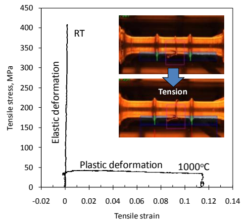
Fig.2 Relationship between tensile applied stress and macroscopic strain at RT and 1000°C.
