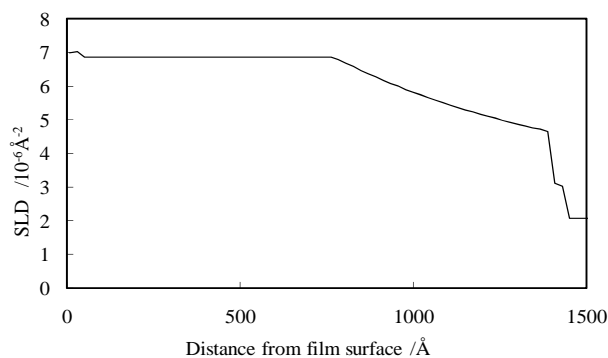
Fig.2 Scattering length density for the DLC ( 50\text{CD}_4, 50\text{H}_2 ) film.
