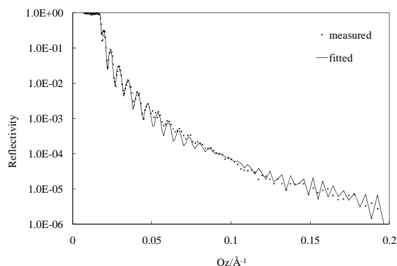
Fig.1 Neutron reflectivity for DLC ( 50\text{CD}_4, 50\text{H}_2 ) film.
